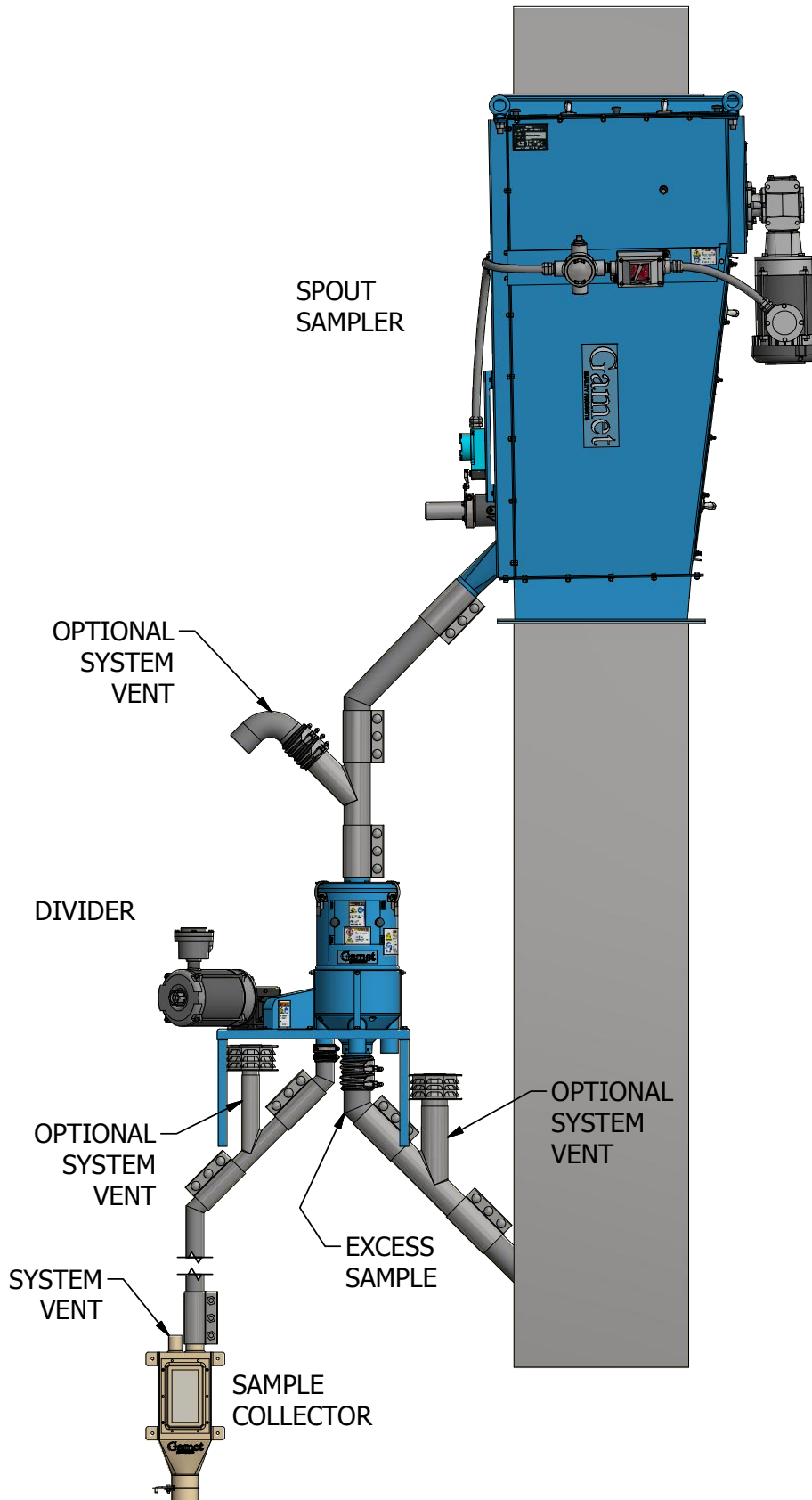
GCD Installation Drawing
