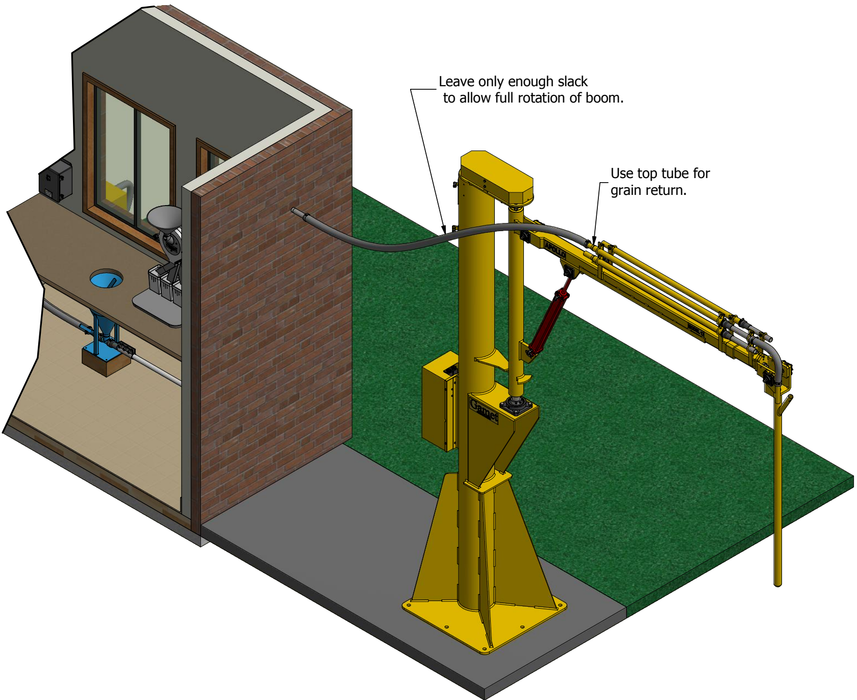
GTA1 Installation Drawing
