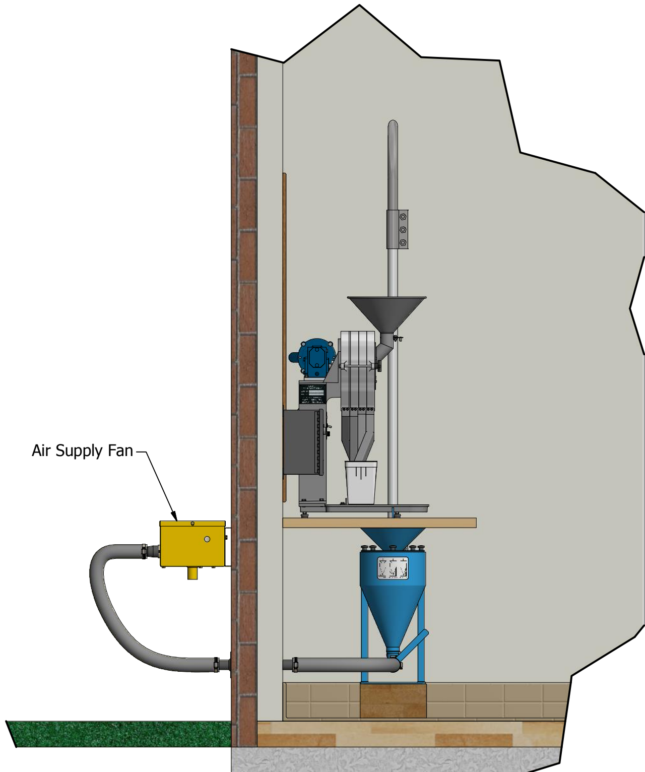
GTA1 Installation Drawing
