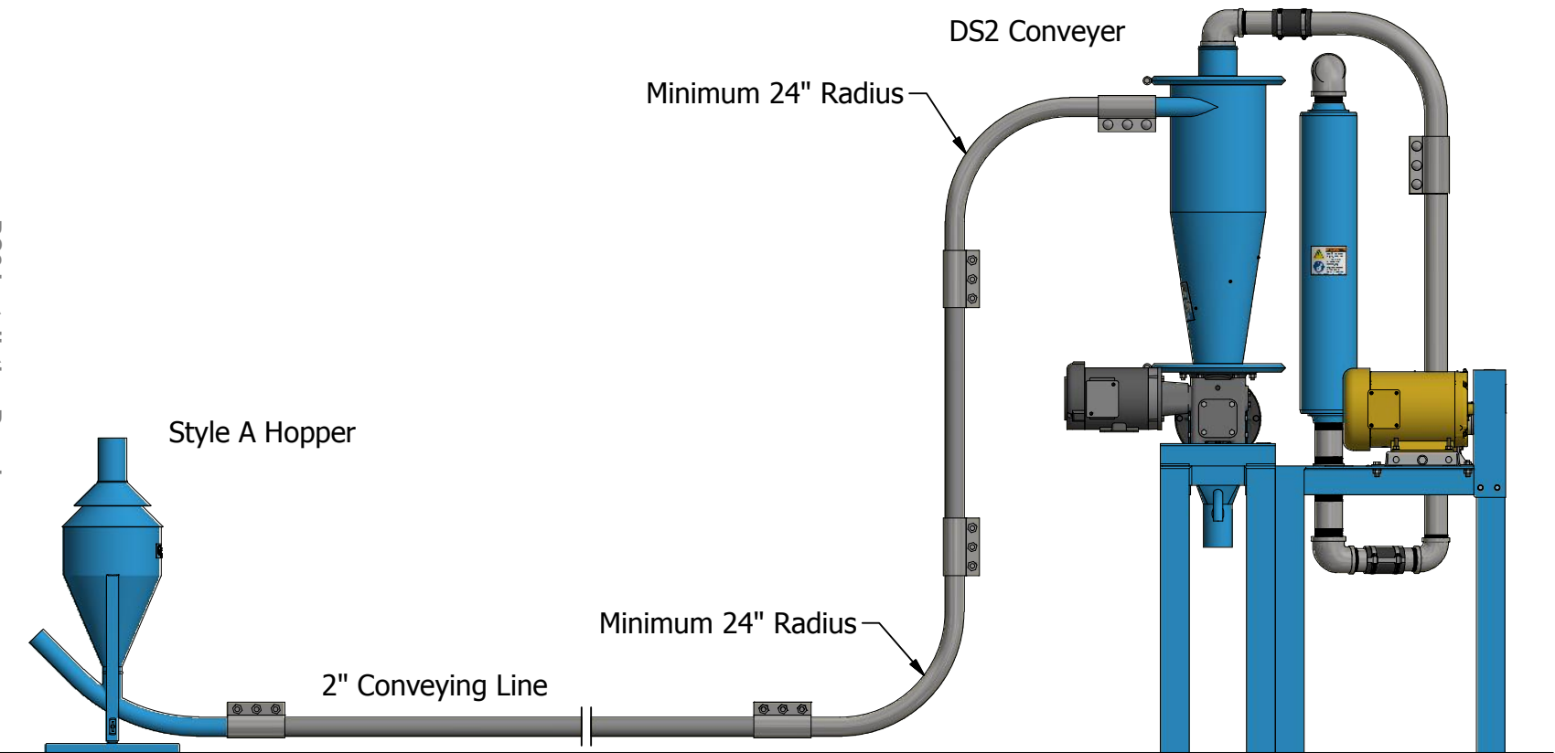
DS2 Installation Drawing
