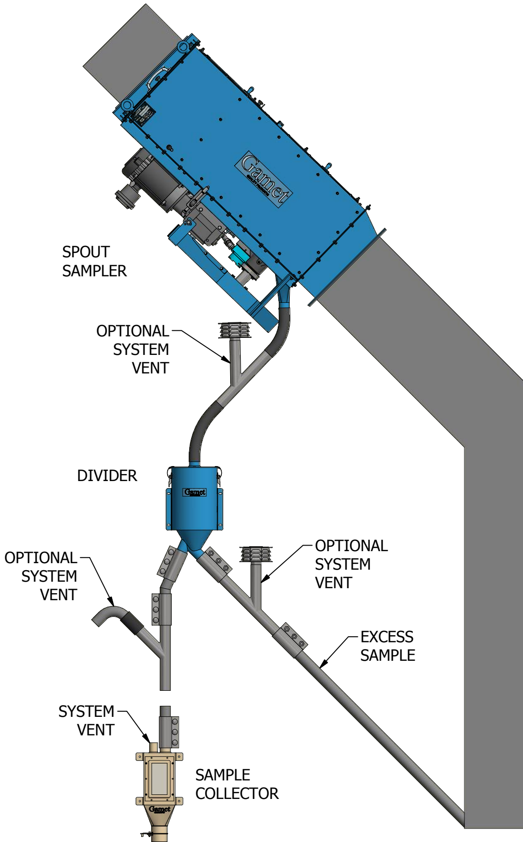
GDGD Installation Drawing
