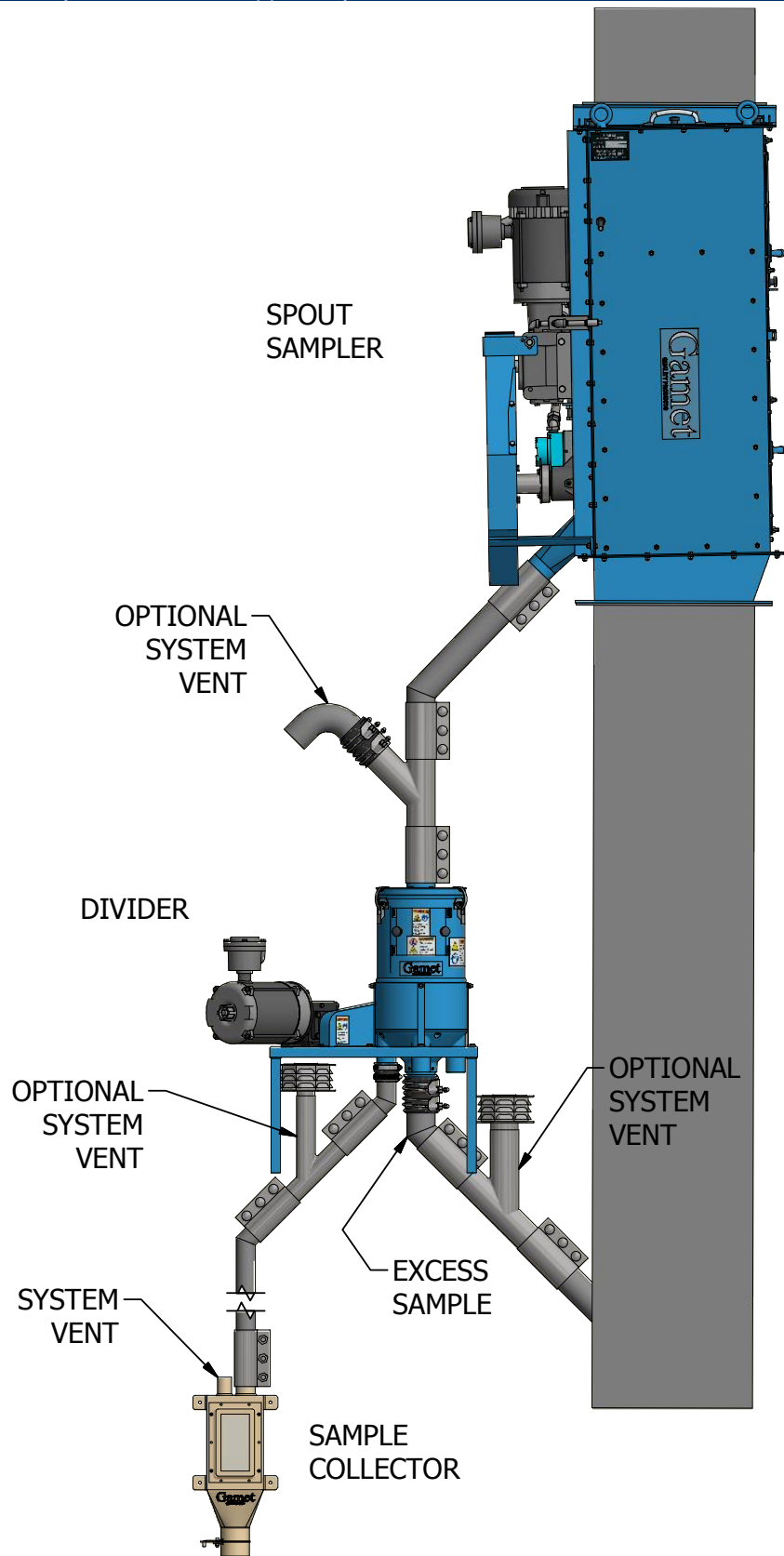
GDCD Installation Drawing
